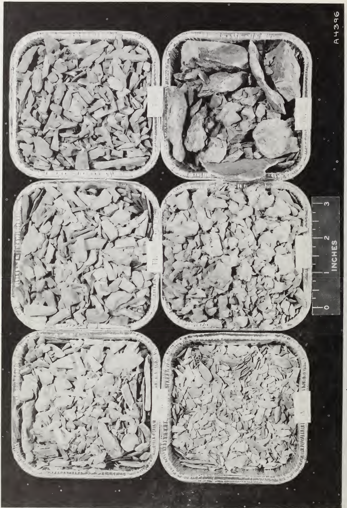
Figure 43. Material remaining after slake-durability testing, TN 7-TN 12.
